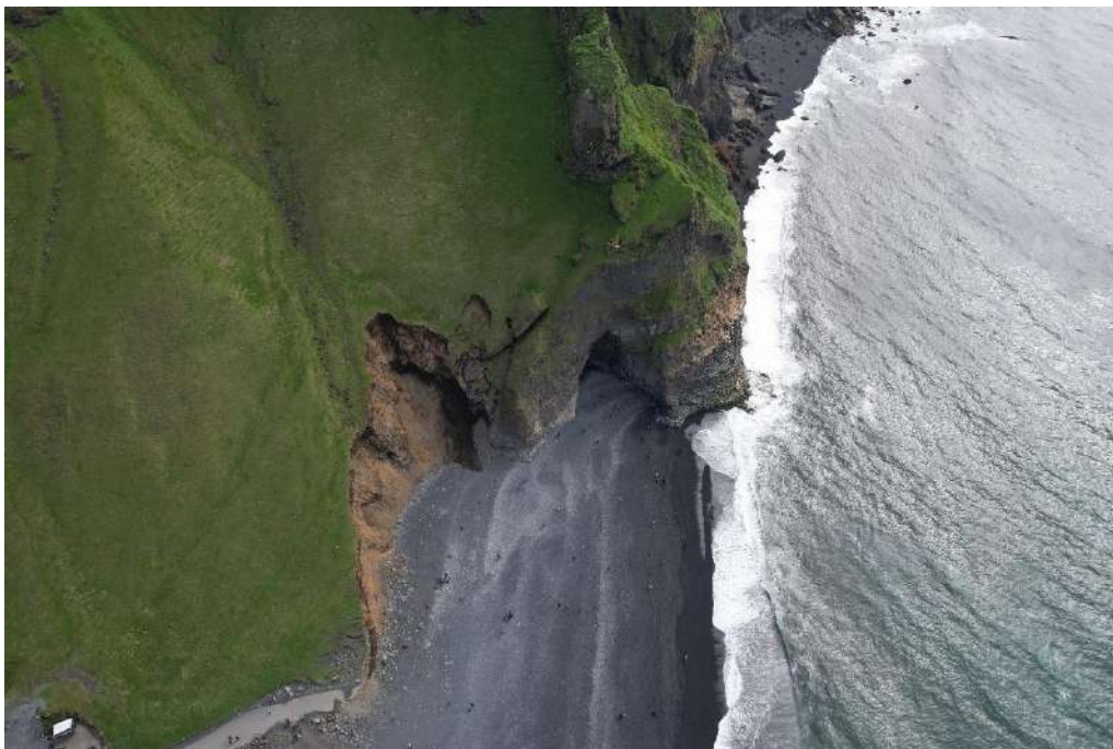
Figure 7 shows the erosional scarp into Reynisfjall, the basalt columns and the cave, along with the beach itself. Before the erosion event in 2026, the beach extended well beyond the basalt columns and the eastern part of the beach was easily accessible.
