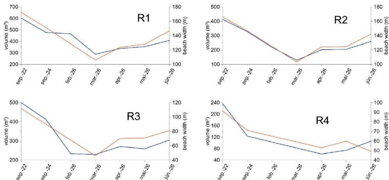
Figure 6 shows the changed in beach width (m) and volume ( m^3 ) of profiles R1-R4. The minimum in beach width and volume was reached in February and March 2026, but since then the beach has been slowly recovering.
